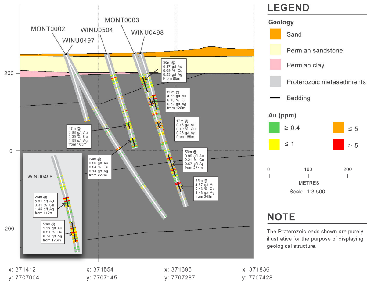
Figure 6: Cross section through Ngapakarra showing the geological model and gold-copper-silver assay intercepts.
