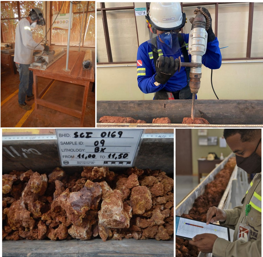
Figure 26 Photographic documentation of the core sample cover removal, crumbling, intervals splitting and logging
