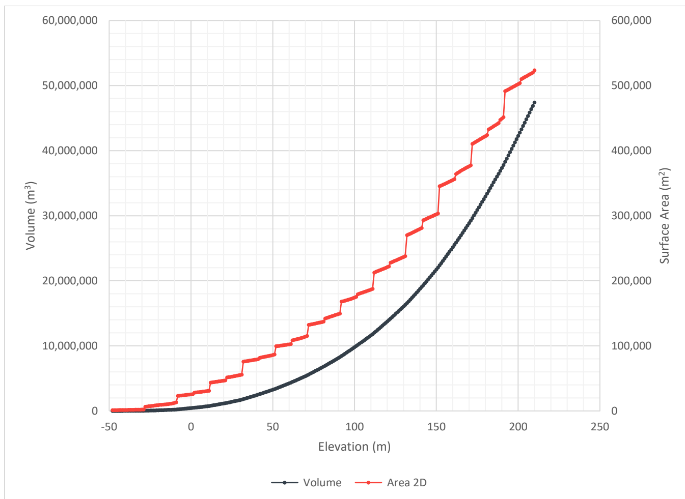
Figure 8: Stage-Volume and Stage-Surface Area Curves for the Final Pit Lake Filling Model
