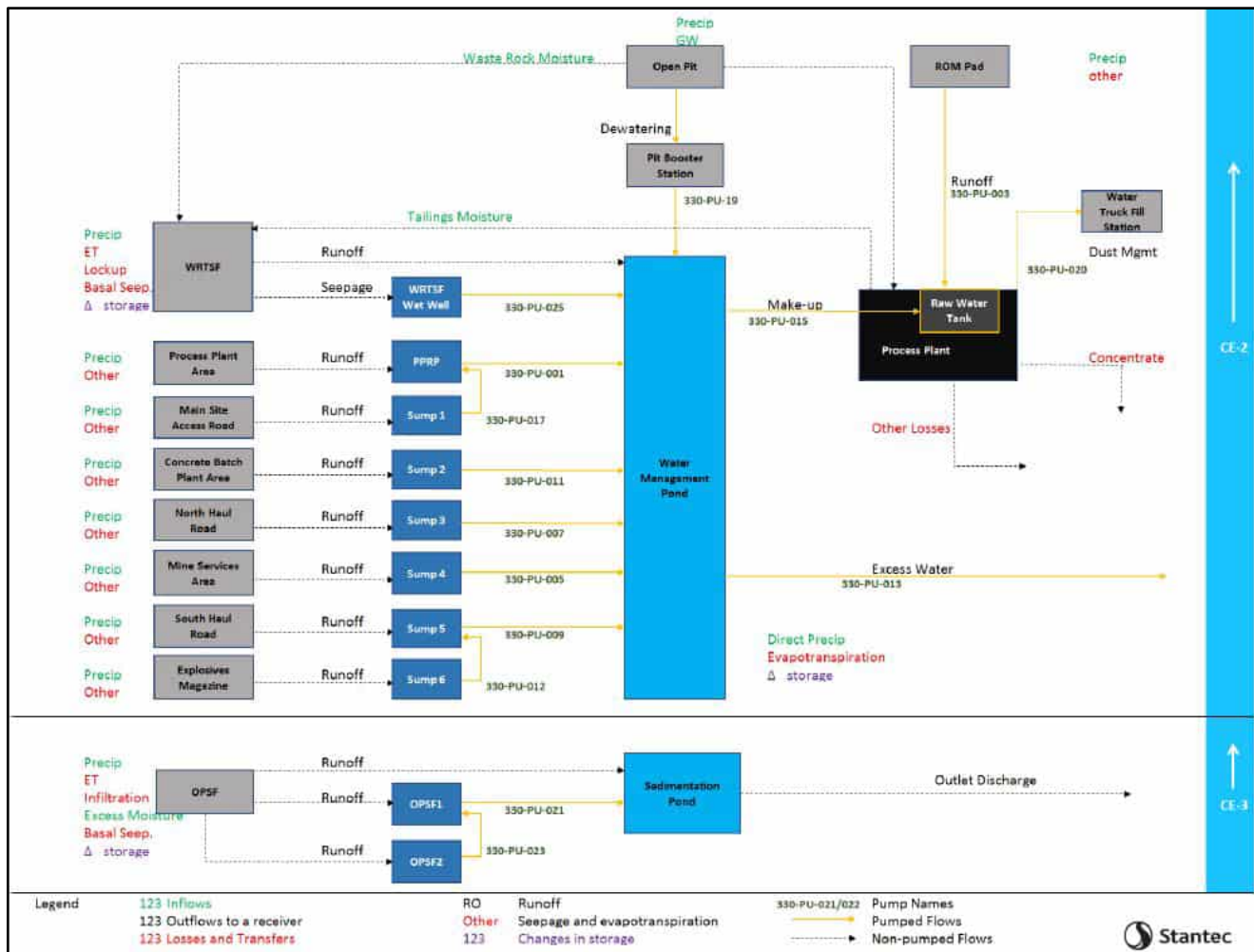
Figure B-3: Site Wide Water Balance Flow Diagram From Initial Water Balance Model (Stantec, 2019)
