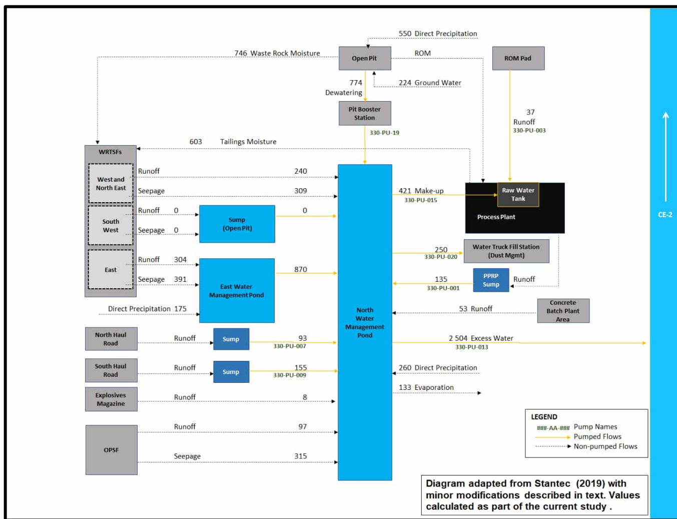
Figure B-9: Water Balance Flow Diagram and Average Flows (m³/day) for Operational Year 3 under Historical Average Climate Conditions
