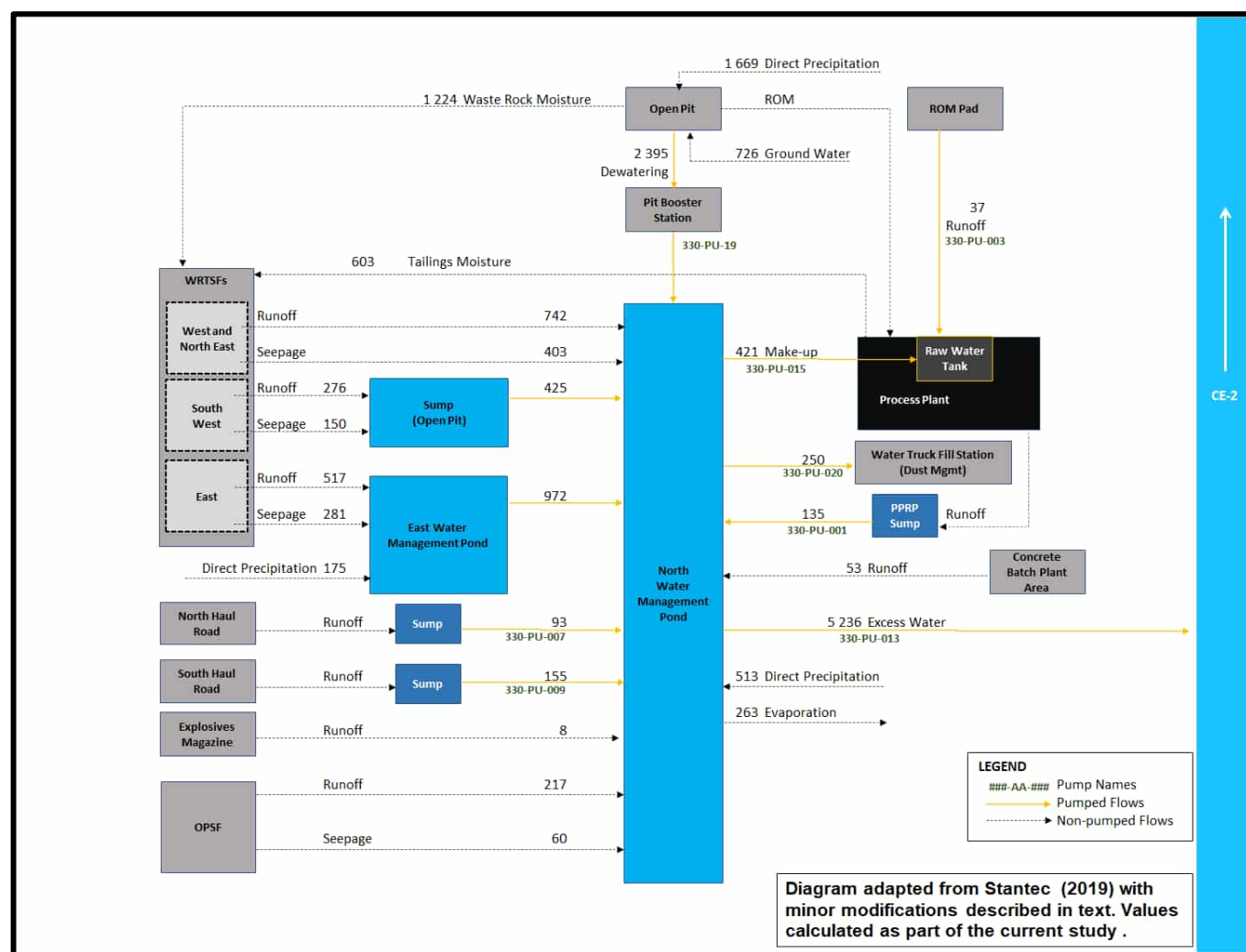
Figure B-10: Water Balance Flow Diagram and Average Flows (m³/day) for Operational Year 9 under Historical Average Climate Conditions
