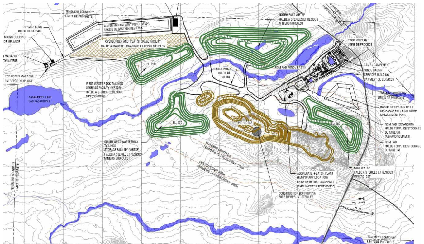
Figure 1: General Site Plan (C Mining Services, 2021)
